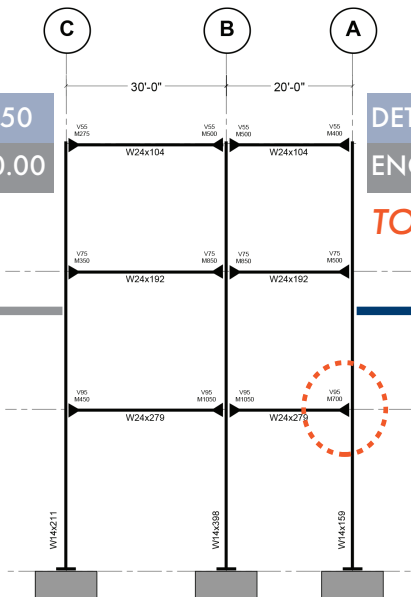
MF-2 ELEVATION ALONG GL 1
